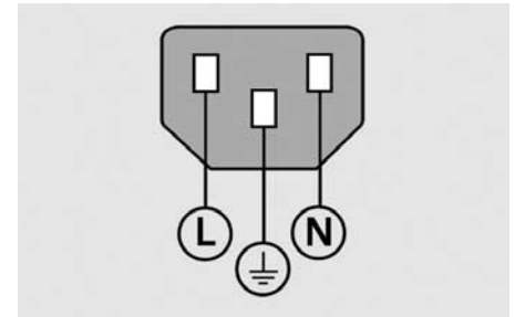
Power cord
